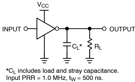
Figure 5. AC Test Circuit
