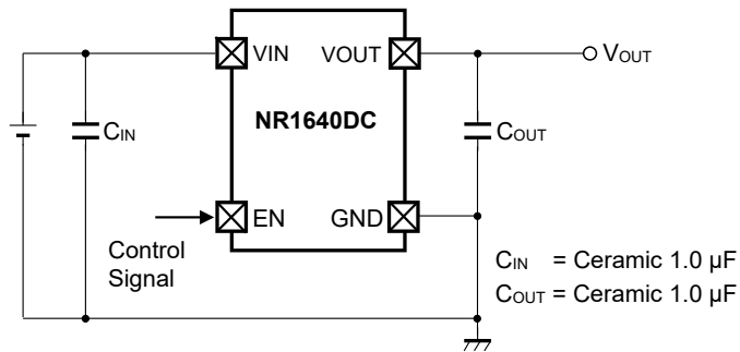
NR1640DC Test Circuit
