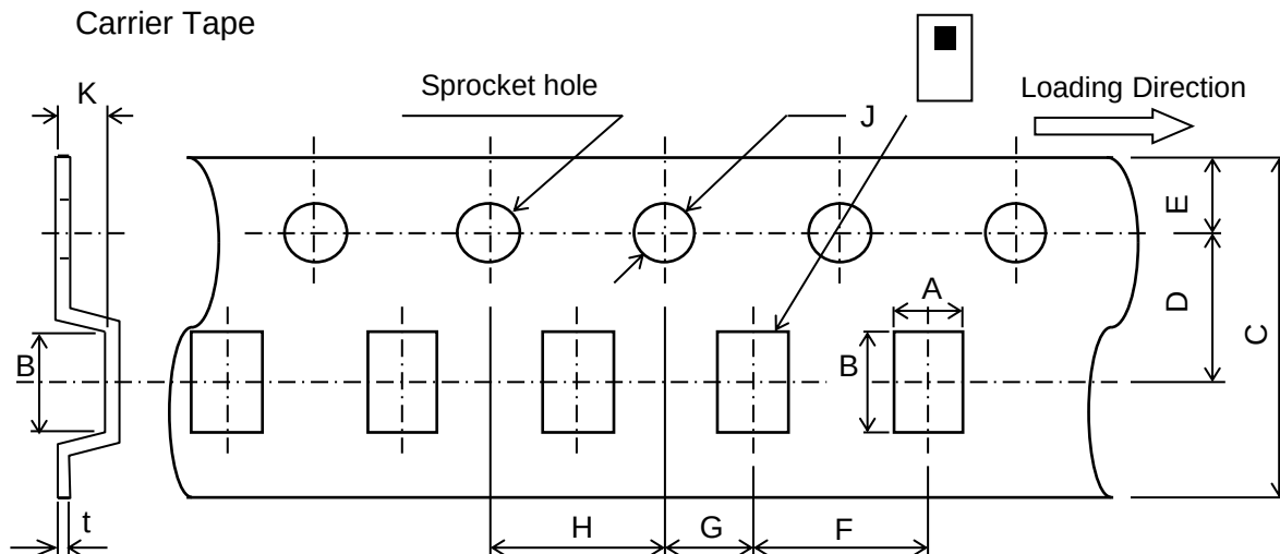
Dimensions (mm)
