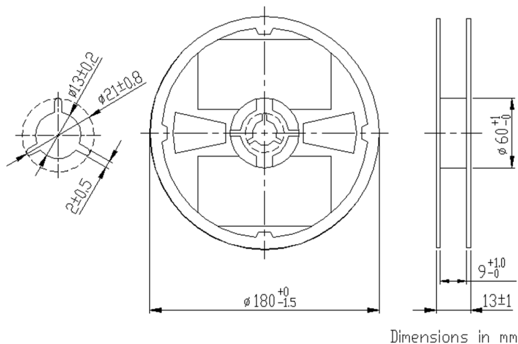
Carrier Tape
