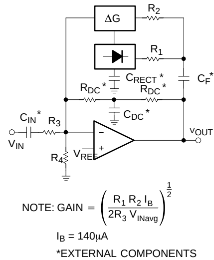
Figure 7. Basic Compressor
