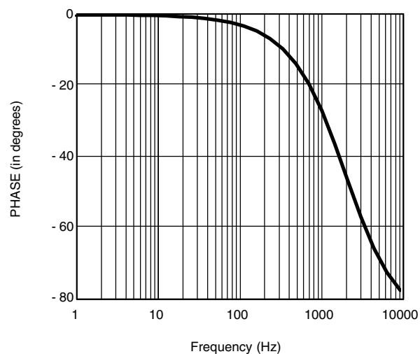
Figure 5. R_L = 6.2 \text{ k}\Omega , C_L = 0.016 \text{ }\mu\text{F}
