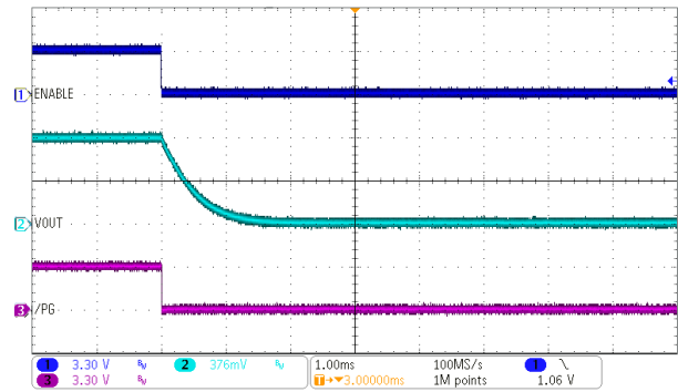
Figure 10-21. Shutdown Using the EN Pin (Discharge Enabled)
