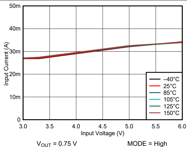
Figure 8-2. Operating Supply Current (Forced PWM)
