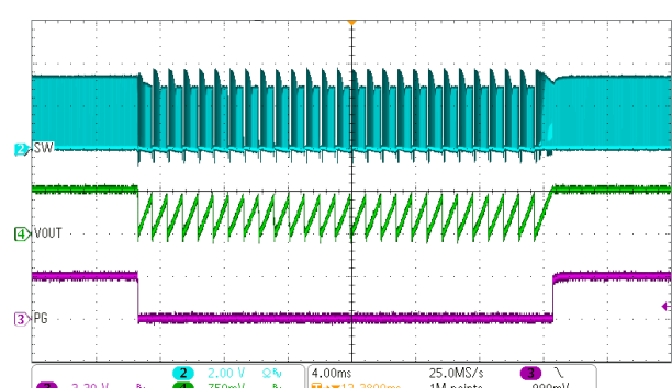
Figure 10-23. Current Limit (Hiccup)
