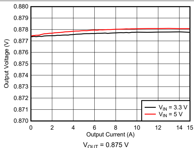
Figure 10-9. Load Regulation
