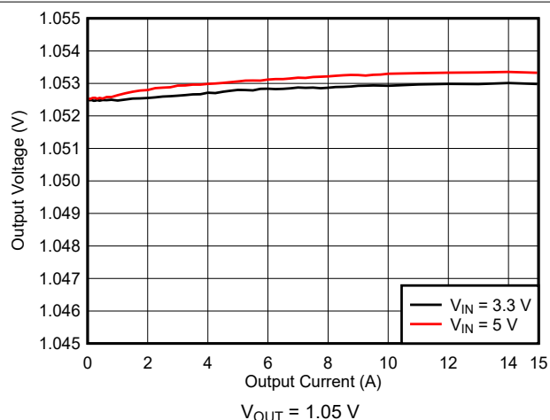
Figure 10-11. Load Regulation
