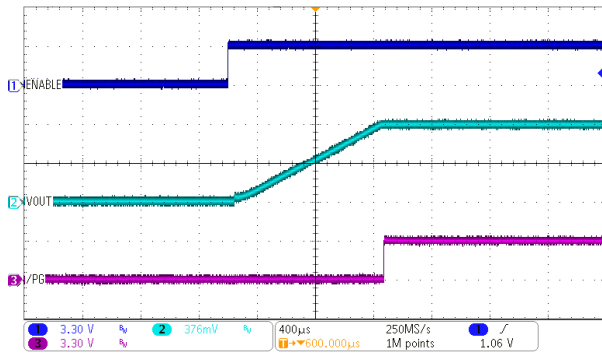
Figure 10-20. Start-Up Using the EN Pin
