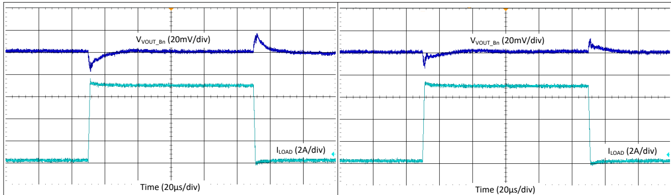
I_{LOAD} = 0.1\text{ A} \rightarrow 7\text{ A} \rightarrow 0.1\text{ A} , T_R = T_F = 1\ \mu\text{s} V_{PVIN\_Bn} = 3.3\text{ V} V_{VOUT\_Bn} = 1\text{ V}
