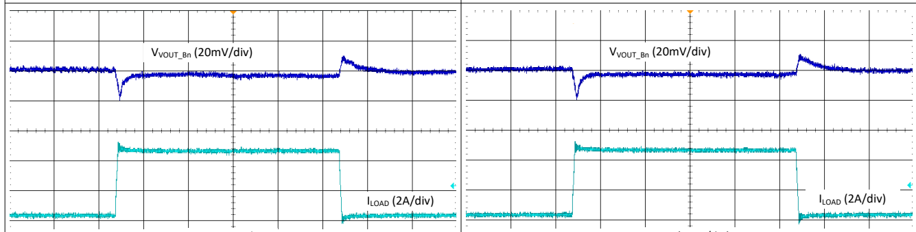
I_{LOAD} = 0.1\text{ A} \rightarrow 5.25\text{ A} \rightarrow 0.1\text{ A} , T_R = T_F = 1\ \mu\text{s} V_{PVIN\_Bn} = 3.3\text{ V} V_{VOUT\_Bn} = 1\text{ V}
